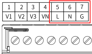
Fig. 2-5 Power Supply Wiring
