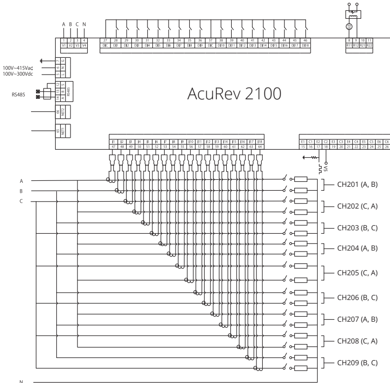
Fig. 2-10 Network Wiring
