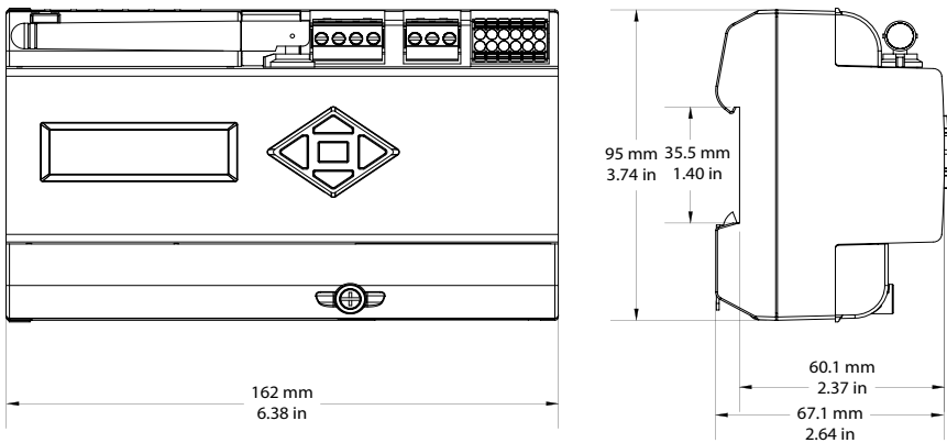
Fig. 2-2 Meter Dimensions (Meter Base, Display, External CTs)
