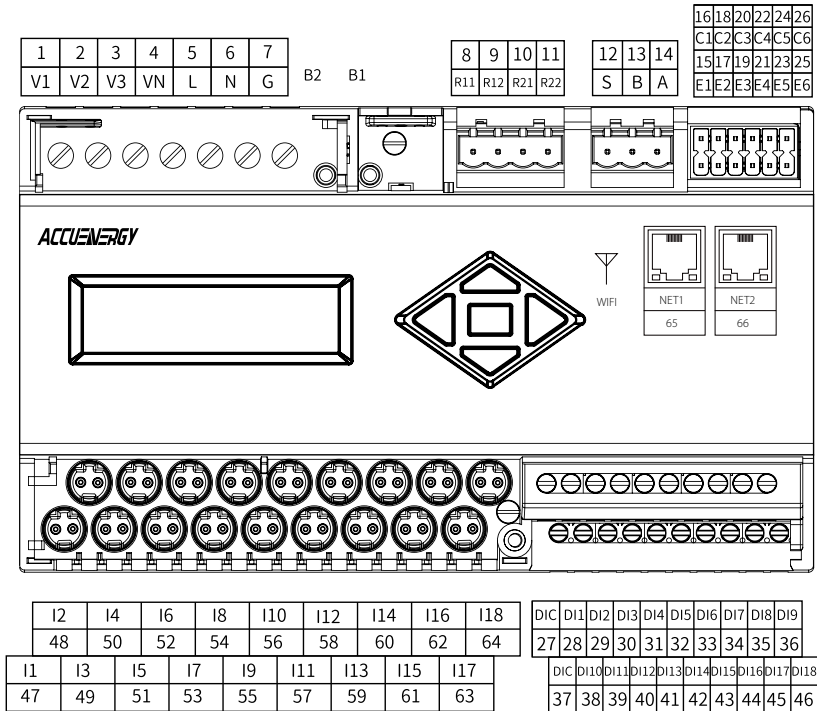
Fig. 2-4 AcuRev 2100 Terminals
