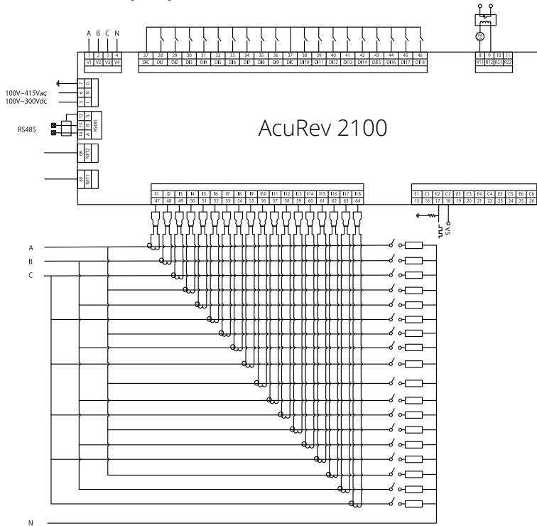
Fig. 2-7 Three-Phase Four-Wire
