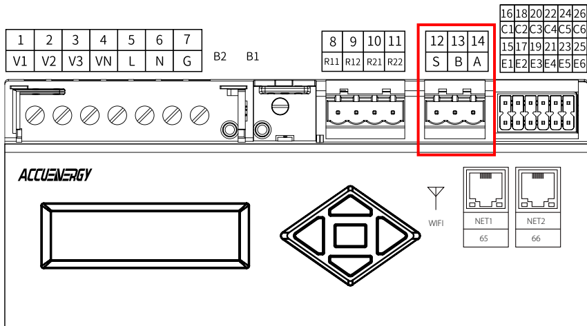
Figure 2-11 Communication Port
